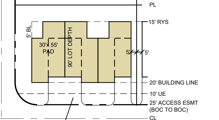
30'x90' MULTIPLEX LOT
