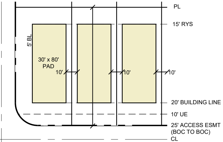
40'x105' SINGLE FAMILY LOT
